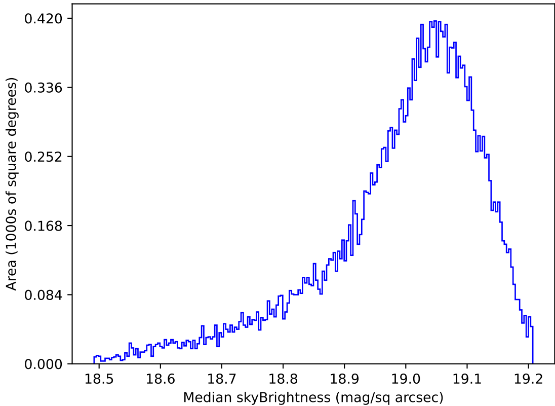
too_elab_heavy_r128_d3_ugrizy_v3.4_10yrs All sky z band: Median skyBrightness
