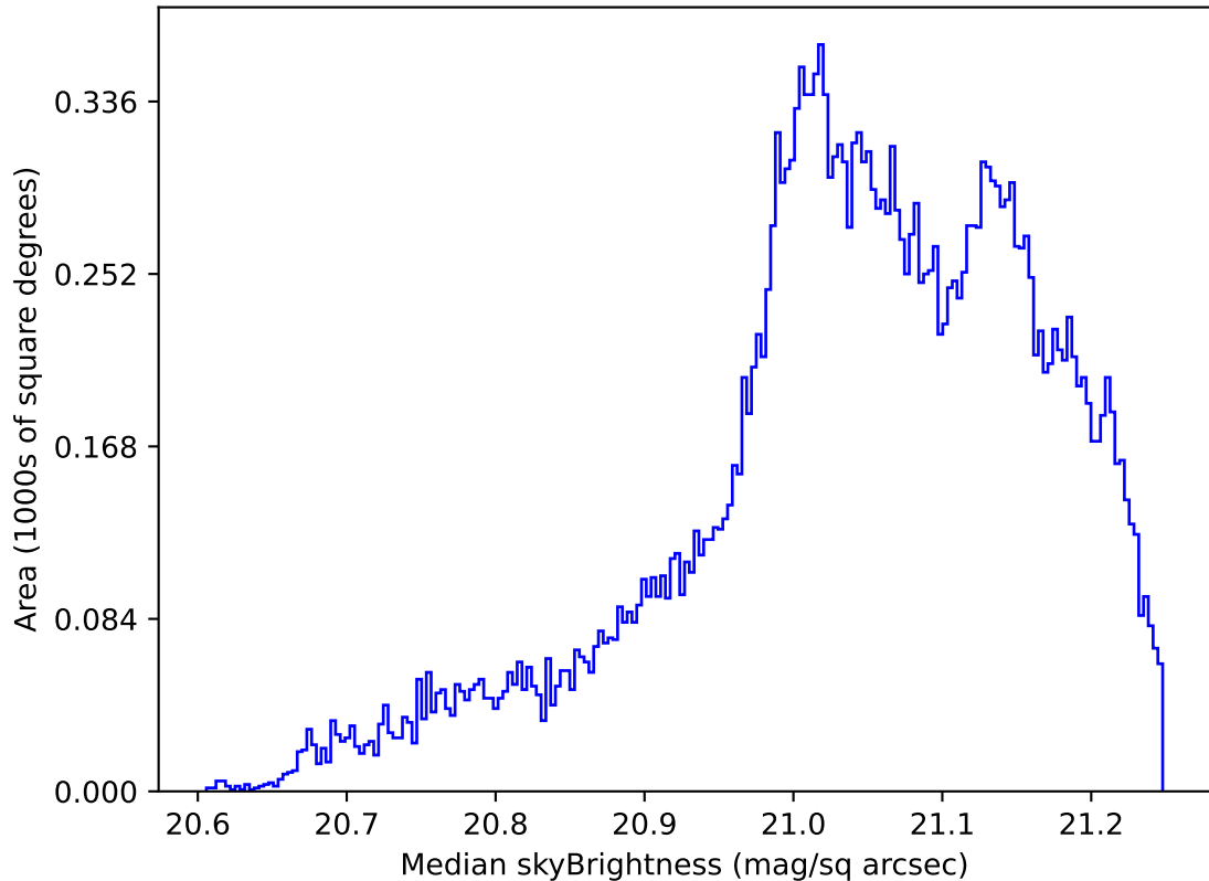
too_elab_heavy_r128_d3_ugrizy_v3.4_10yrs All sky r band: Median skyBrightness
