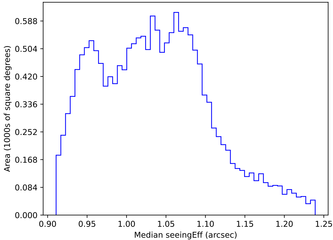
too_elab_heavy_r128_d3_ugrizy_v3.4_10yrs WFD all bands: Median seeingEff
