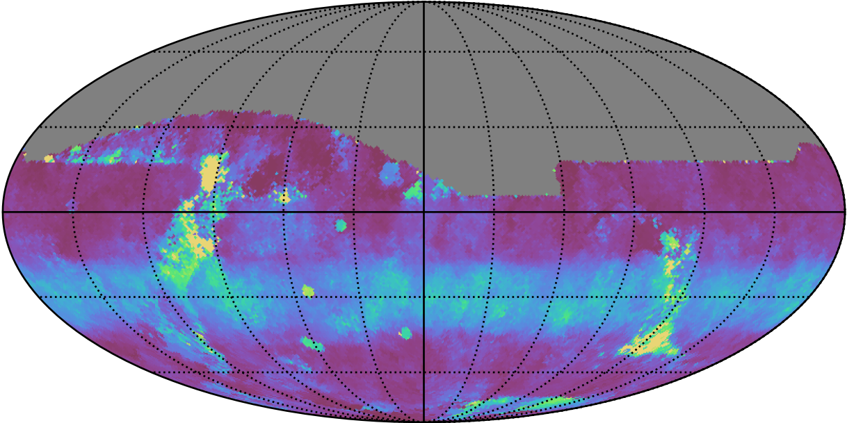
too_elab_heavy_r128_d3_ugrizy_v3.4_10yrs All sky z band: Median normairmass
