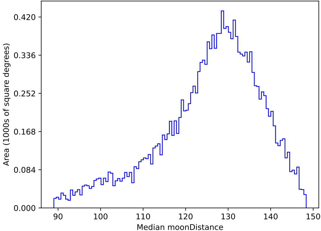
too_elab_heavy_r128_d3_ugrizy_v3.4_10yrs WFD u band: Median moonDistance
