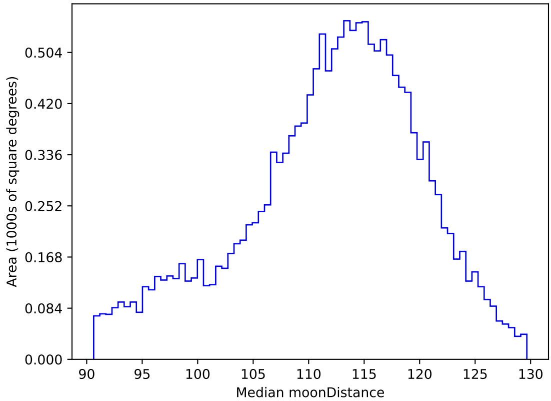
too_elab_heavy_r128_d3_ugrizy_v3.4_10yrs WFD r band: Median moonDistance
