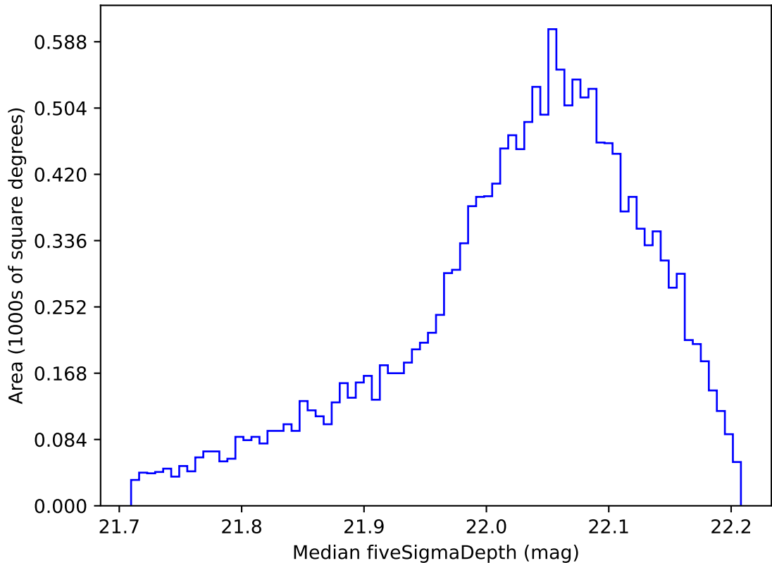
too_elab_heavy_r128_d3_ugrizy_v3.4_10yrs WFD y band: Median fiveSigmaDepth
