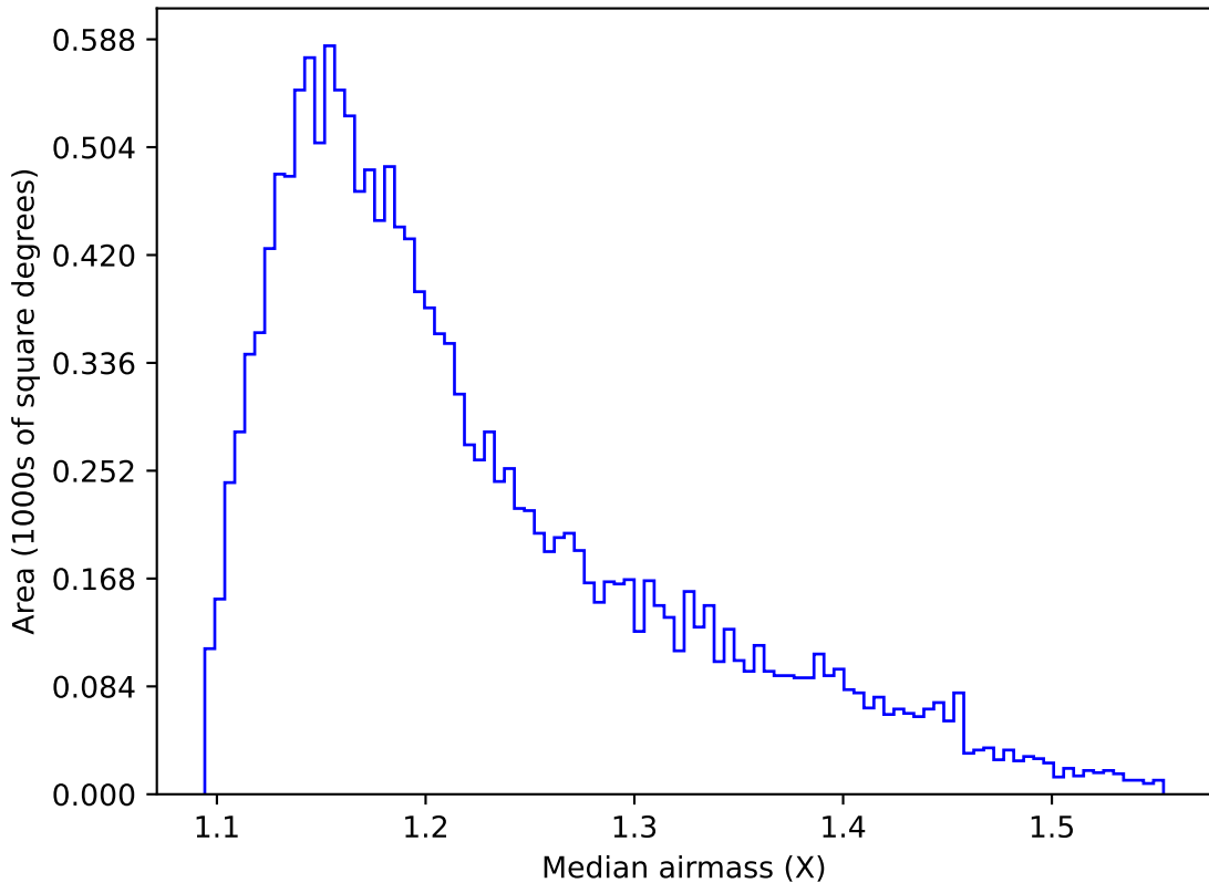
too_elab_heavy_r128_d3_ugrizy_v3.4_10yrs WFD g band: Median airmass
