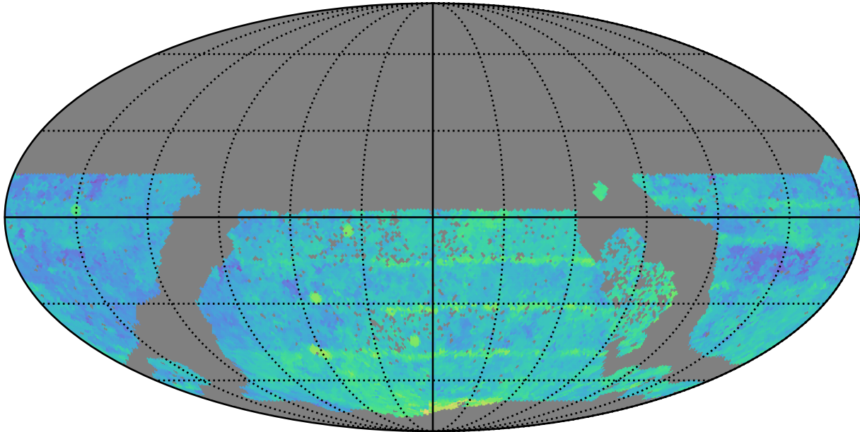
too_elab_heavy_r128_d3_ugrizy_v3.4_10yrs WFD z band: Median Season Length
