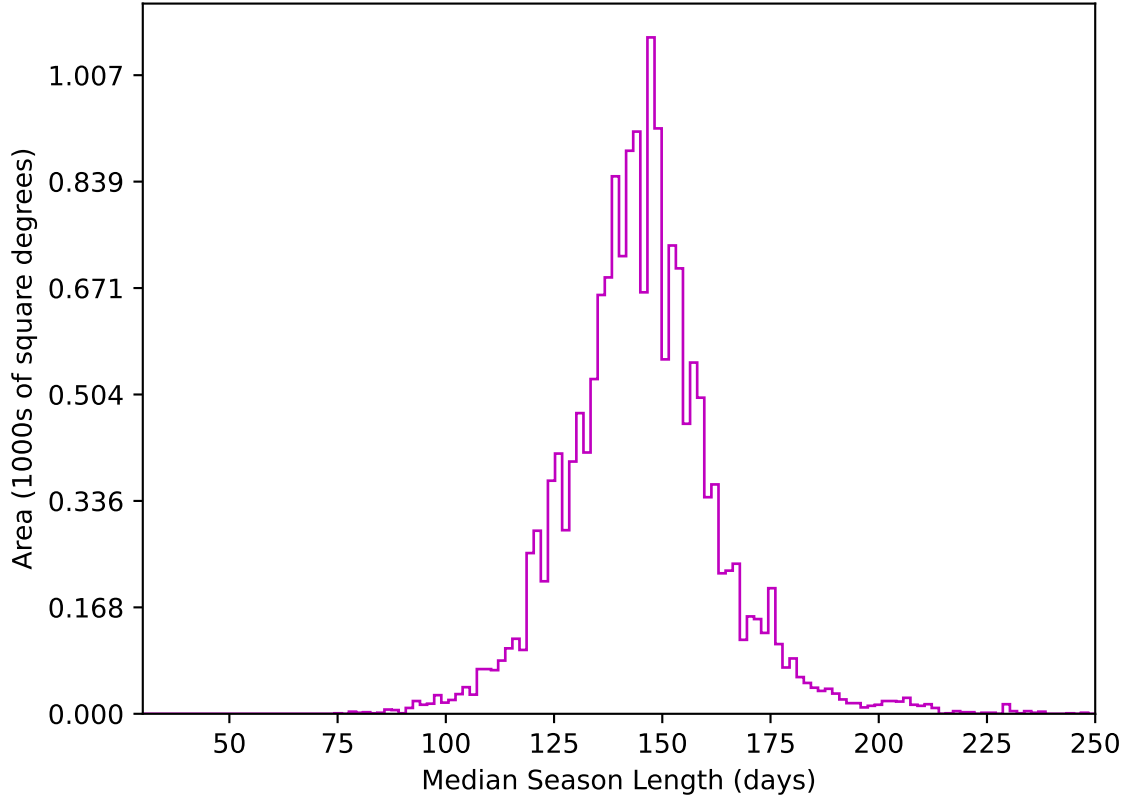
too_elab_heavy_r128_d3_ugrizy_v3.4_10yrs WFD z band: Median Season Length
