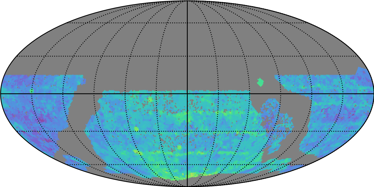
too_elab_heavy_r128_d3_ugrizy_v3.4_10yrs WFD y band: Median Season Length
