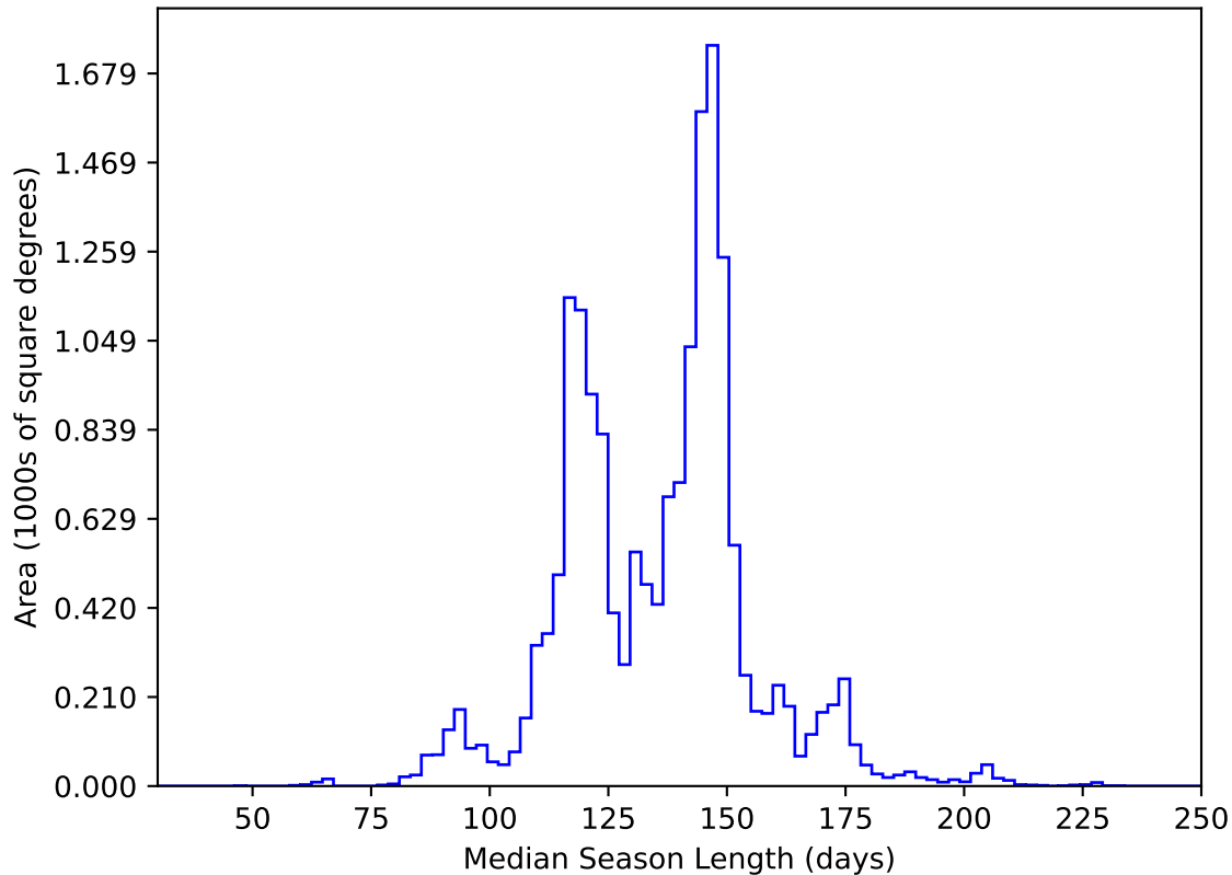
too_elab_heavy_r128_d3_ugrizy_v3.4_10yrs WFD y band: Median Season Length
