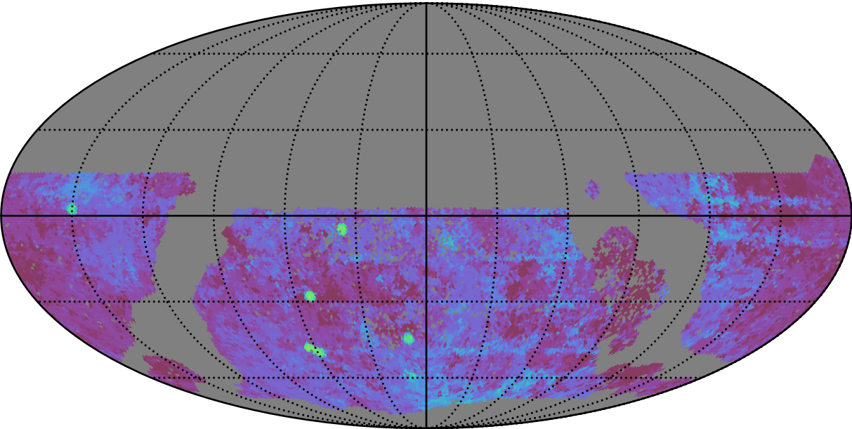
too_elab_heavy_r128_d3_ugrizy_v3.4_10yrs WFD u band: Median Season Length
