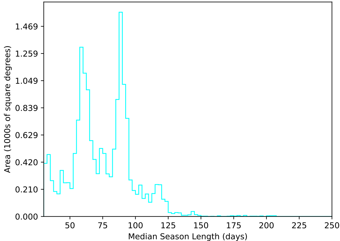
too_elab_heavy_r128_d3_ugrizy_v3.4_10yrs WFD u band: Median Season Length
