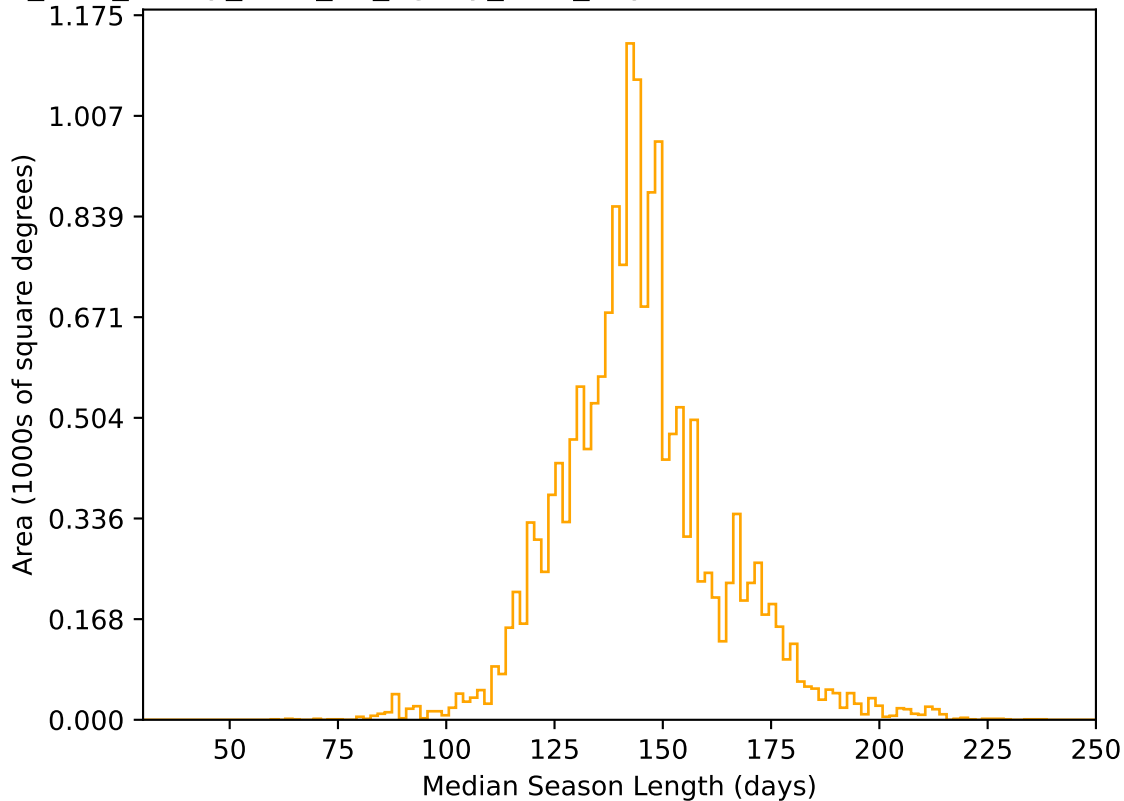
too_elab_heavy_r128_d3_ugrizy_v3.4_10yrs WFD r band: Median Season Length
