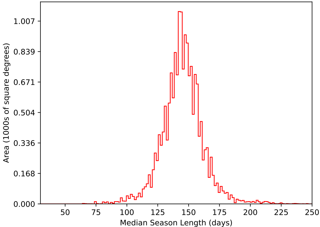
too_elab_heavy_r128_d3_ugrizy_v3.4_10yrs WFD i band: Median Season Length
