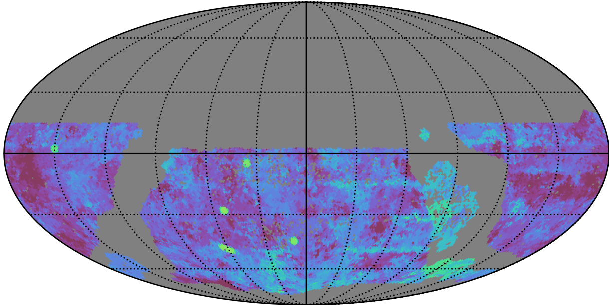
too_elab_heavy_r128_d3_ugrizy_v3.4_10yrs WFD g band: Median Season Length
