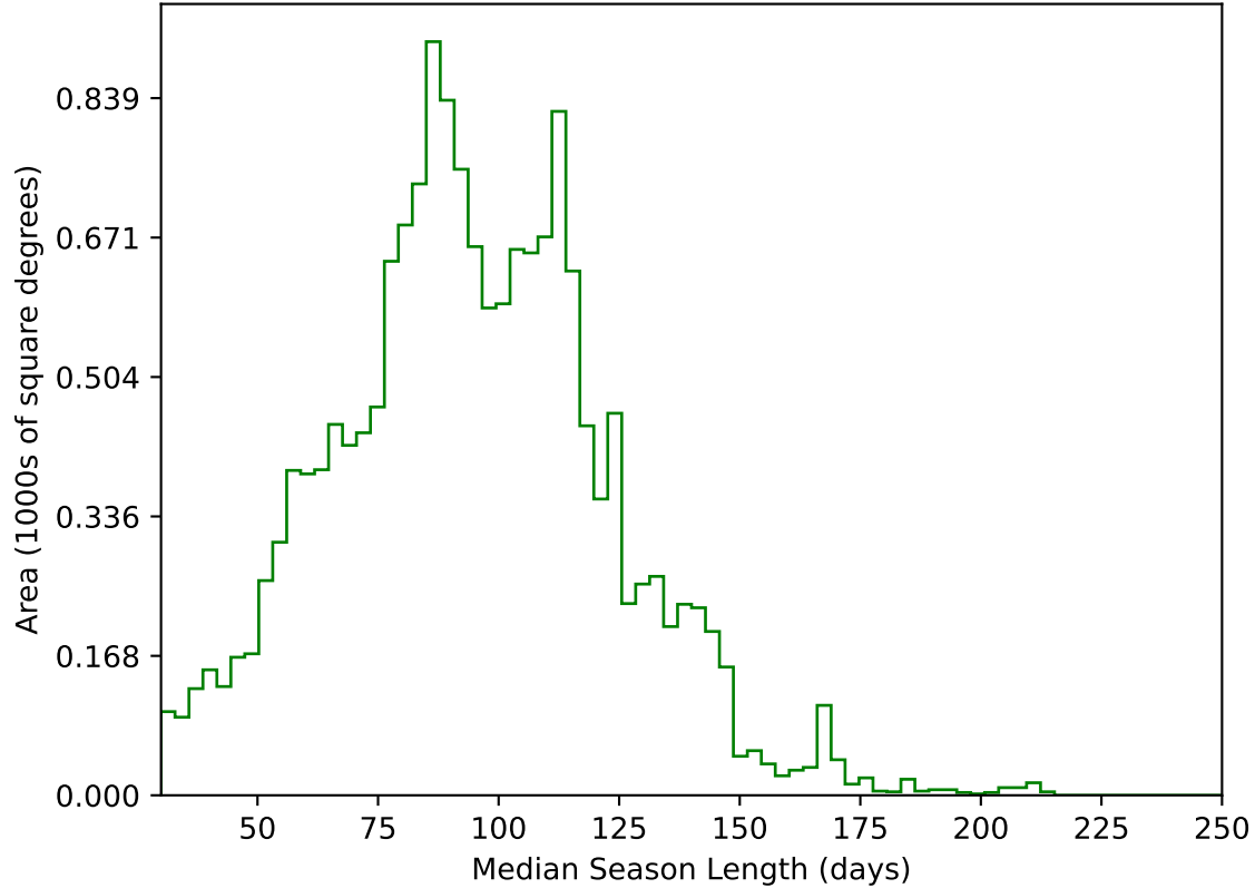
too_elab_heavy_r128_d3_ugrizy_v3.4_10yrs WFD g band: Median Season Length
