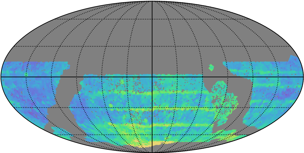
too_elab_heavy_r128_d3_ugrizy_v3.4_10yrs WFD all bands: Median Season Length
