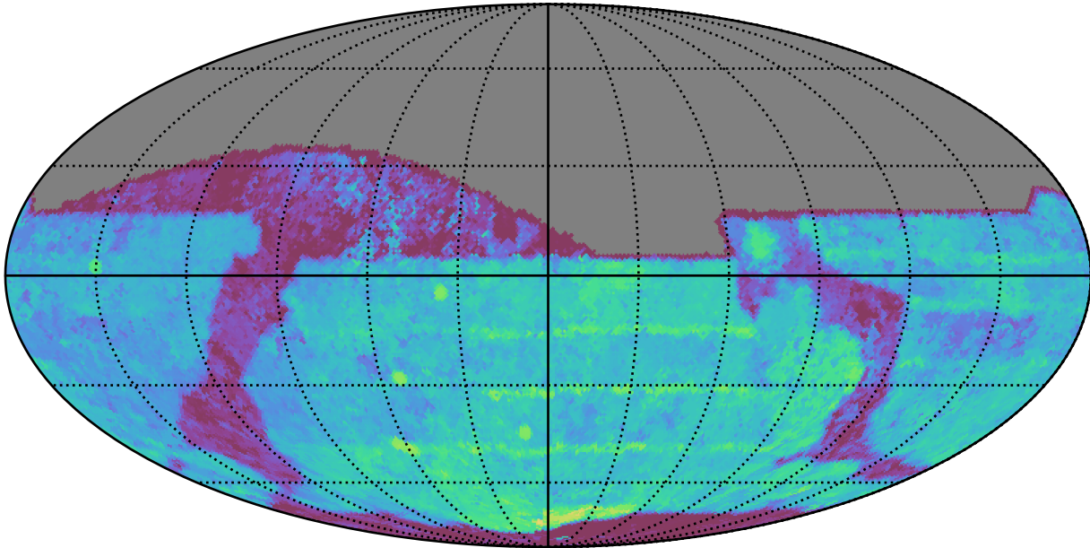
too_elab_heavy_r128_d3_ugrizy_v3.4_10yrs All sky z band: Median Season Length
