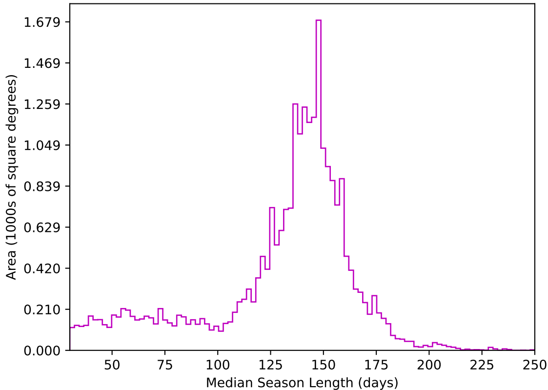
too_elab_heavy_r128_d3_ugrizy_v3.4_10yrs All sky z band: Median Season Length
