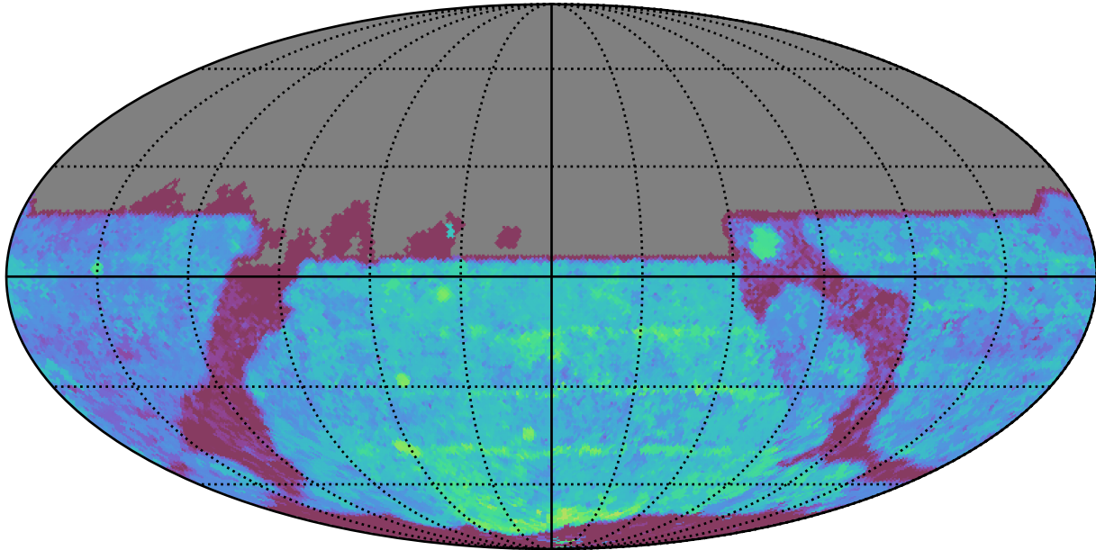
too_elab_heavy_r128_d3_ugrizy_v3.4_10yrs All sky y band: Median Season Length
