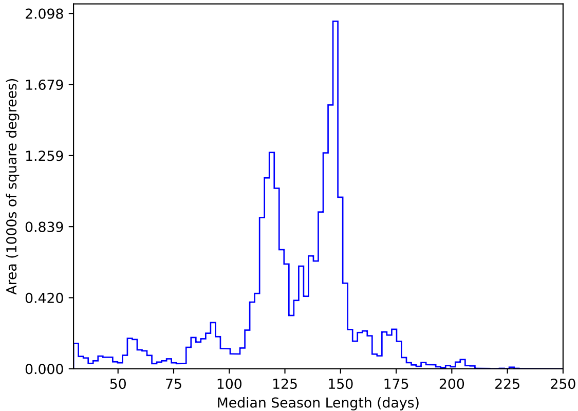
too_elab_heavy_r128_d3_ugrizy_v3.4_10yrs All sky y band: Median Season Length
