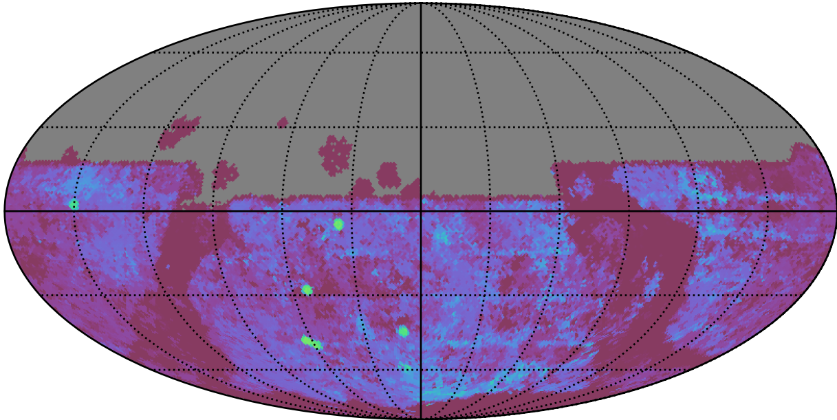
too_elab_heavy_r128_d3_ugrizy_v3.4_10yrs All sky u band: Median Season Length
