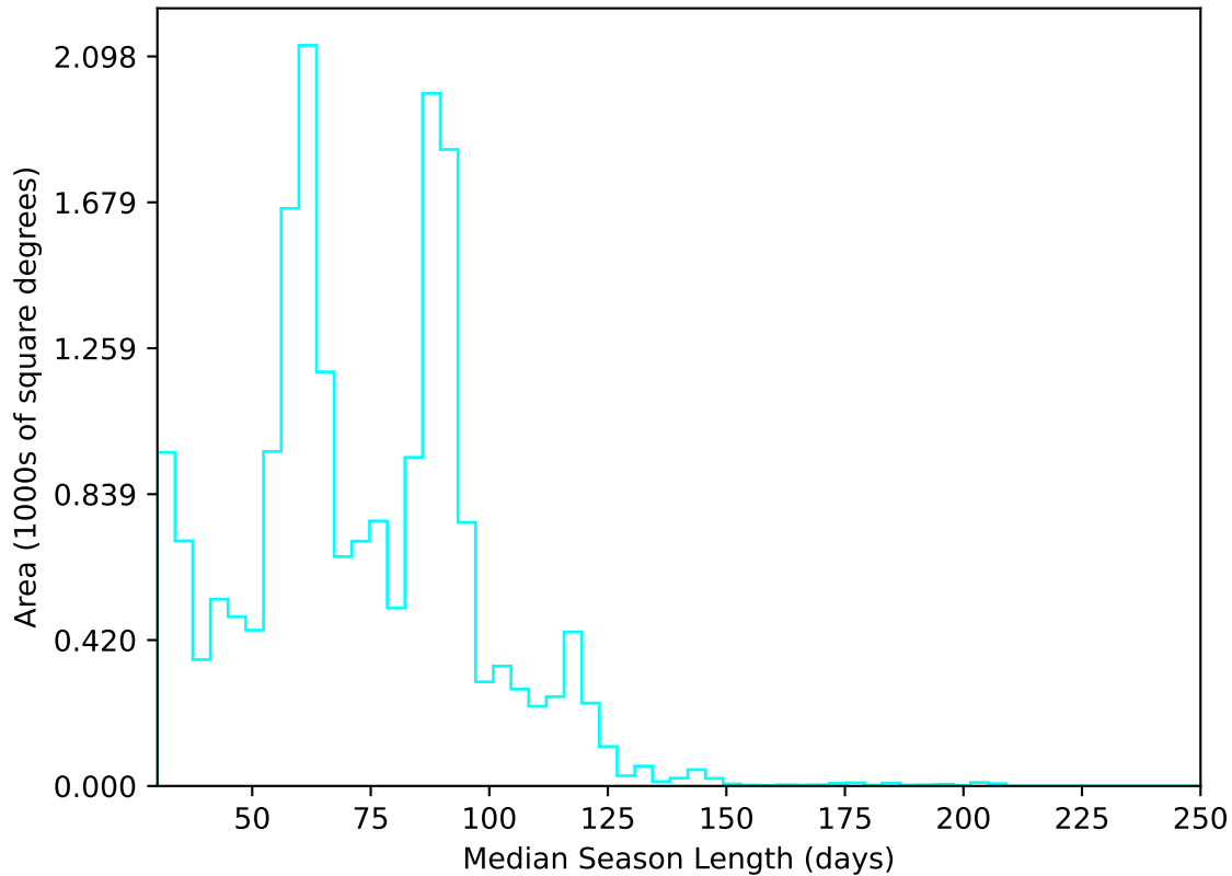
too_elab_heavy_r128_d3_ugrizy_v3.4_10yrs All sky u band: Median Season Length
