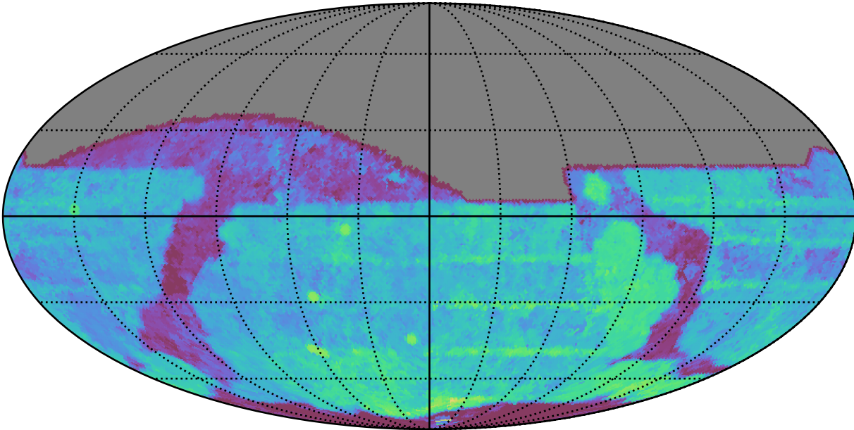
too_elab_heavy_r128_d3_ugrizy_v3.4_10yrs All sky r band: Median Season Length
