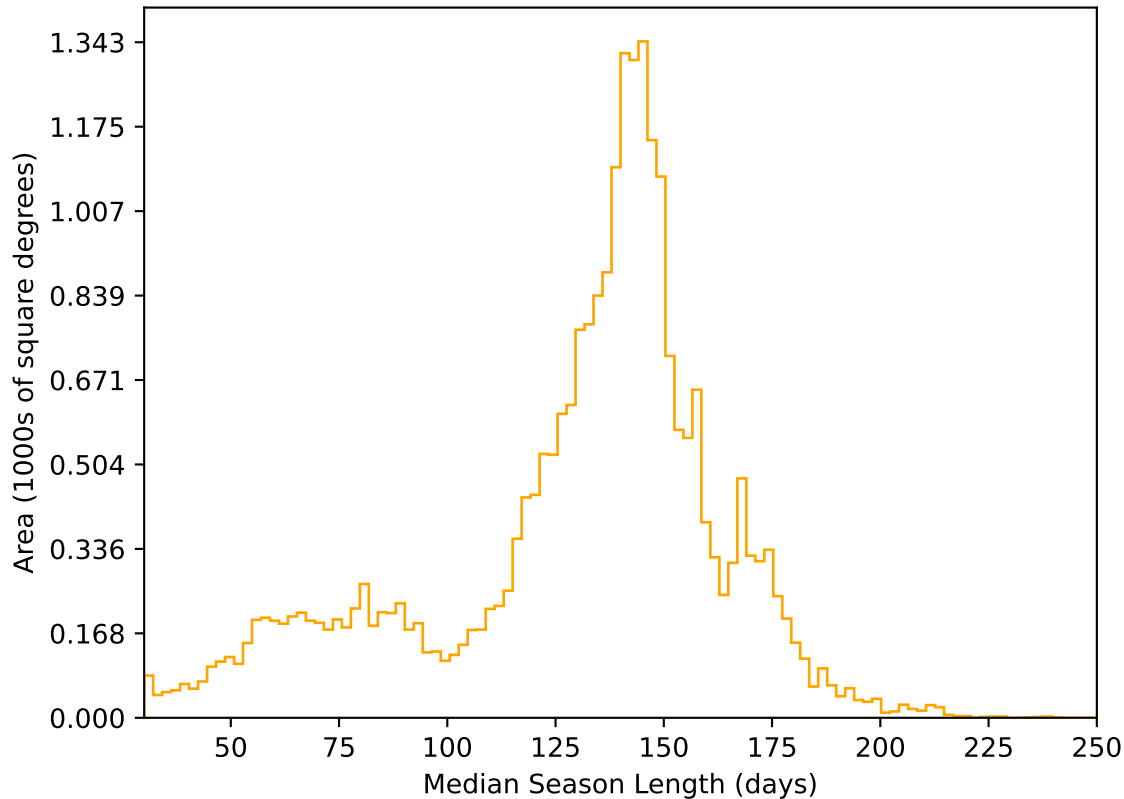
too_elab_heavy_r128_d3_ugrizy_v3.4_10yrs All sky r band: Median Season Length
