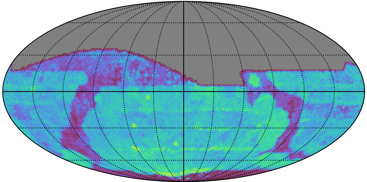
too_elab_heavy_r128_d3_ugrizy_v3.4_10yrs All sky i band: Median Season Length
