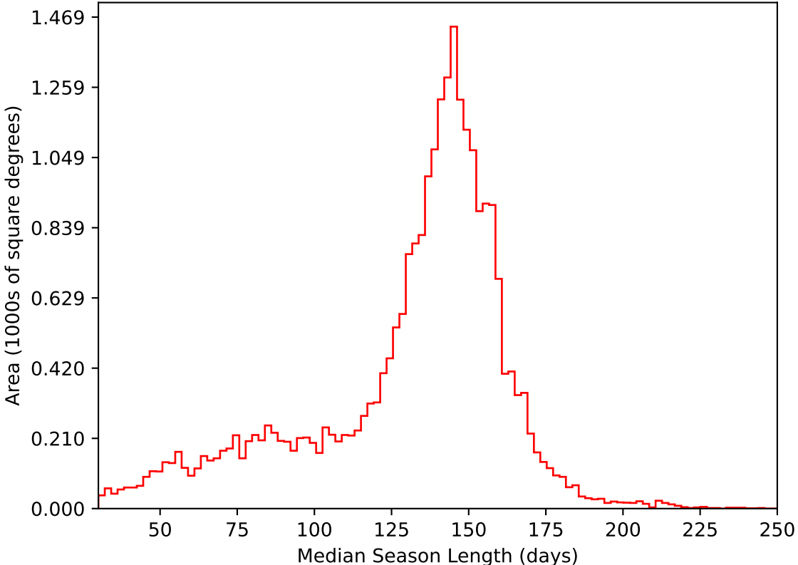
too_elab_heavy_r128_d3_ugrizy_v3.4_10yrs All sky i band: Median Season Length
