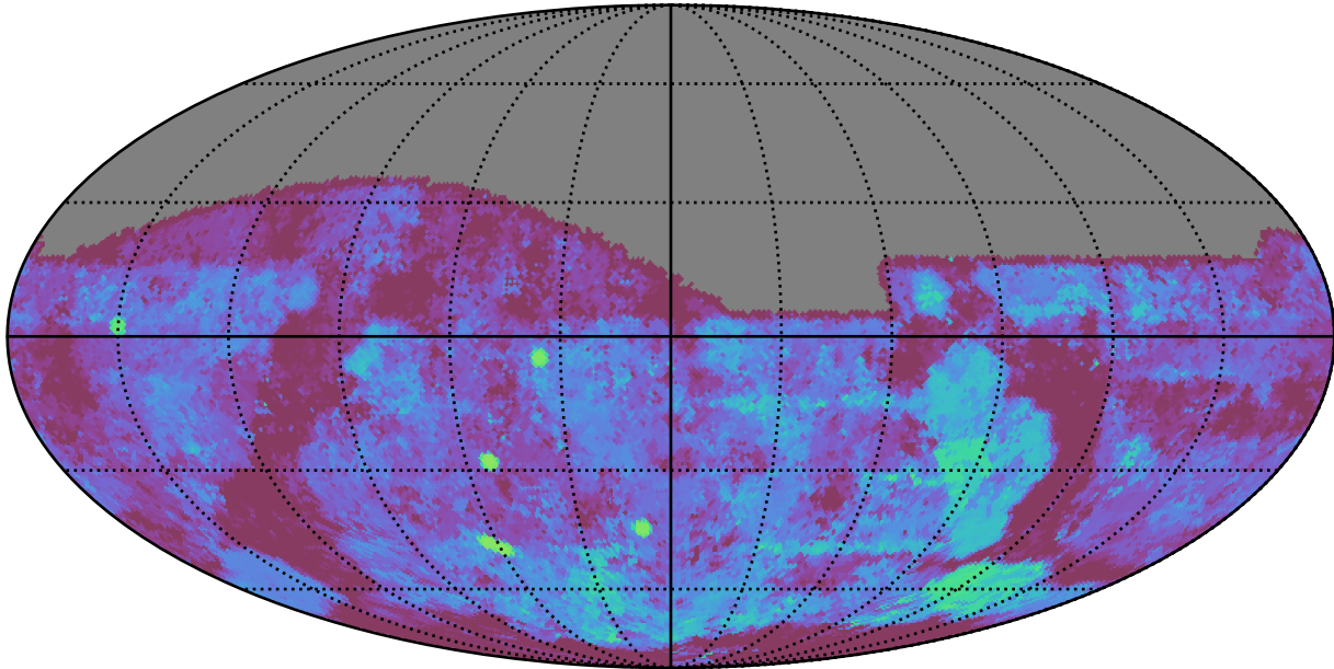
too_elab_heavy_r128_d3_ugrizy_v3.4_10yrs All sky g band: Median Season Length
