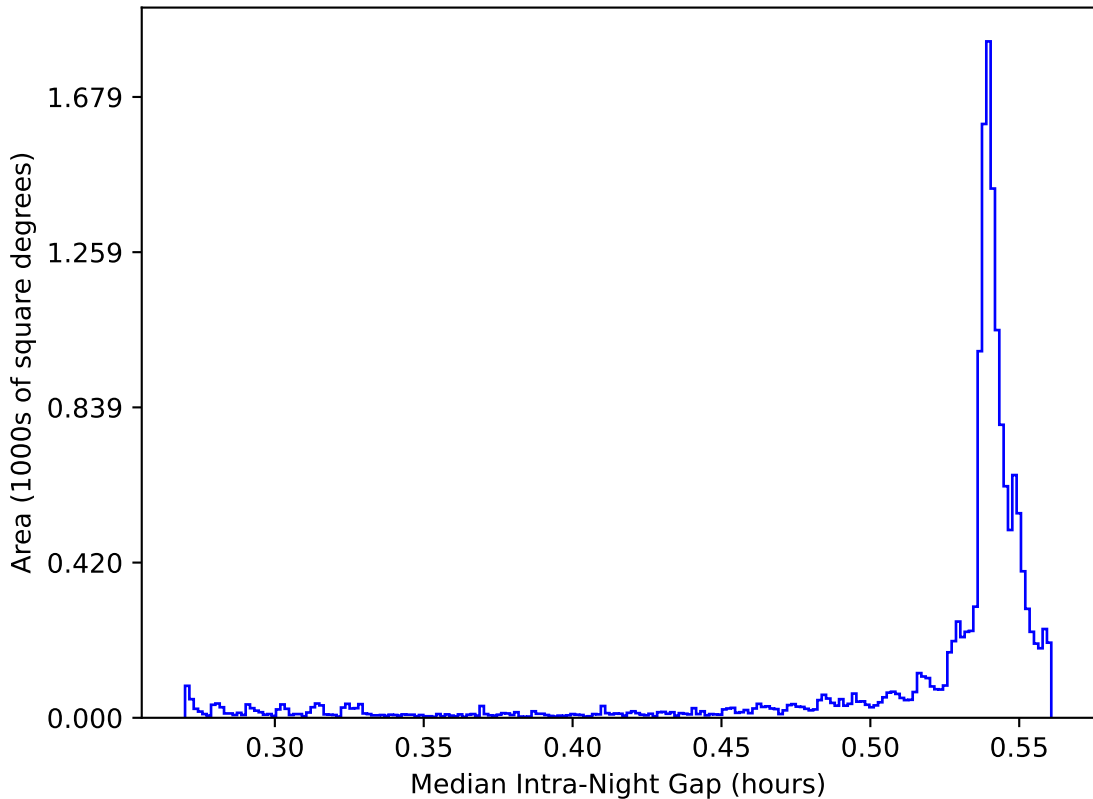
too_elab_heavy_r128_d3_ugrizy_v3.4_10yrs WFD: Median Intra-Night Gap
