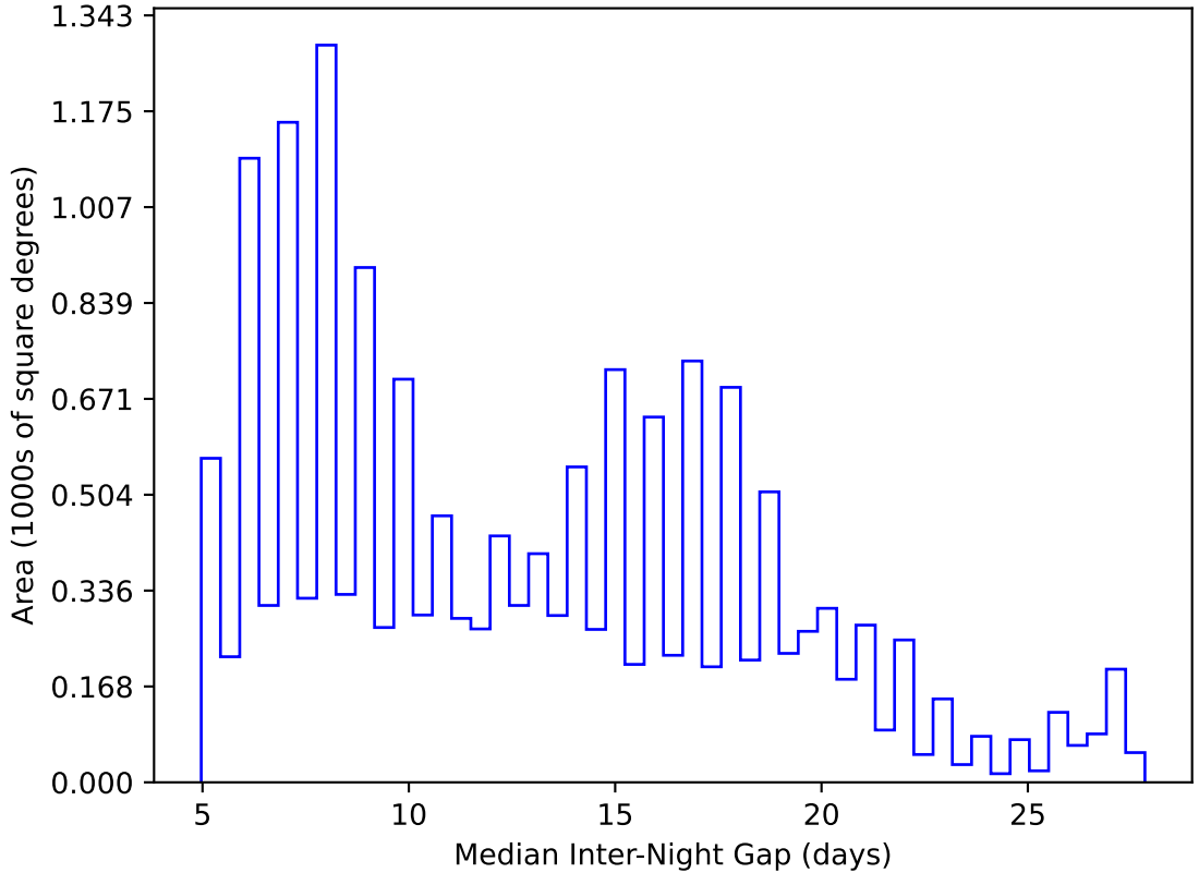
too_elab_heavy_r128_d3_ugrizy_v3.4_10yrs WFD y band: Median Inter-Night Gap
