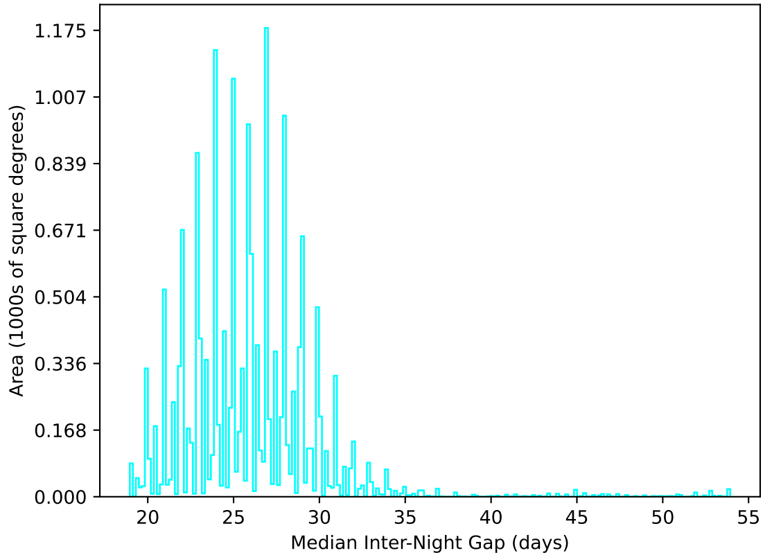
too_elab_heavy_r128_d3_ugrizy_v3.4_10yrs WFD u band: Median Inter-Night Gap
