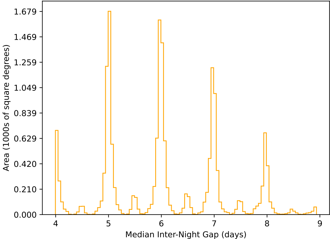
too_elab_heavy_r128_d3_ugrizy_v3.4_10yrs WFD r band: Median Inter-Night Gap
