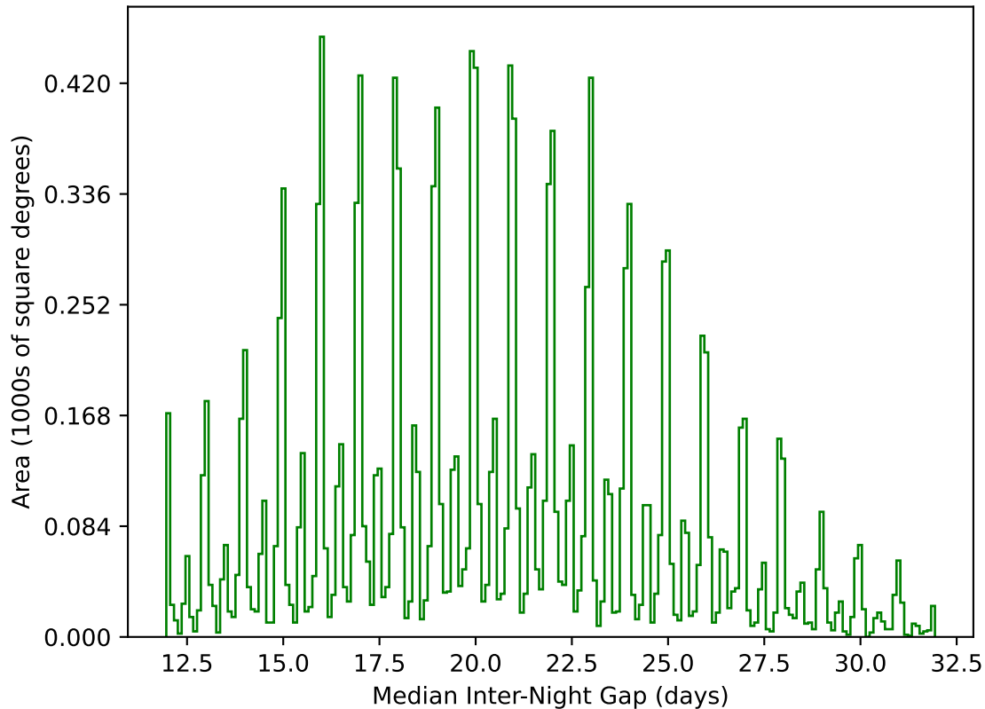
too_elab_heavy_r128_d3_ugrizy_v3.4_10yrs WFD g band: Median Inter-Night Gap
