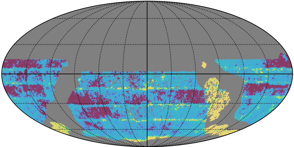
too_elab_heavy_r128_d3_ugrizy_v3.4_10yrs WFD all bands: Median Inter-Night Gap
