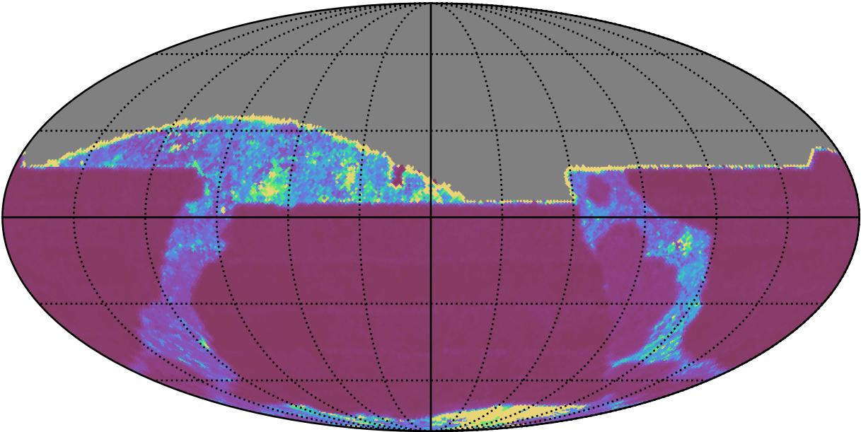
too_elab_heavy_r128_d3_ugrizy_v3.4_10yrs All sky z band: Median Inter-Night Gap
