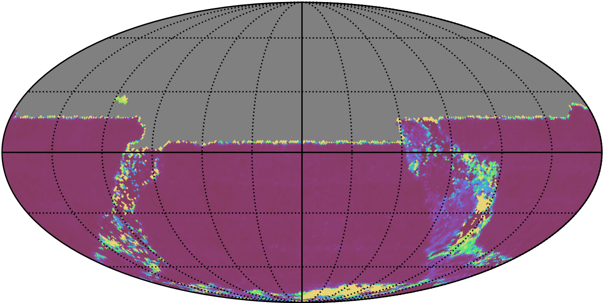
too_elab_heavy_r128_d3_ugrizy_v3.4_10yrs All sky u band: Median Inter-Night Gap
