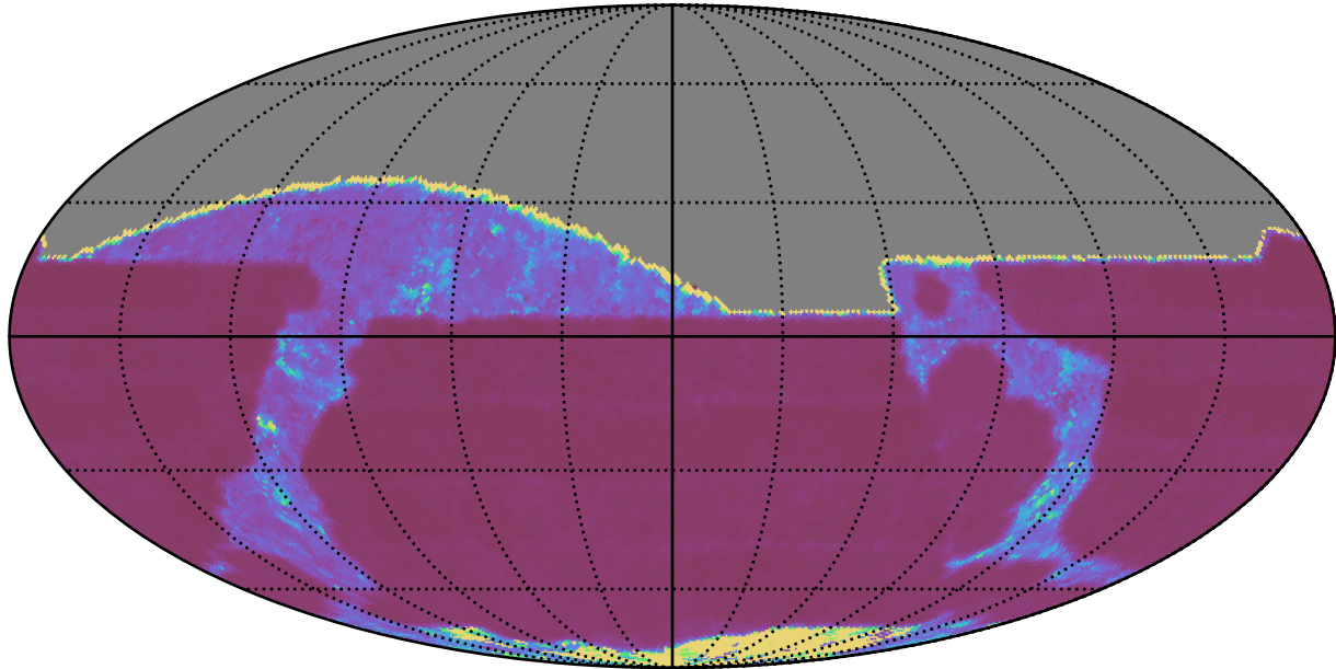
too_elab_heavy_r128_d3_ugrizy_v3.4_10yrs All sky r band: Median Inter-Night Gap
