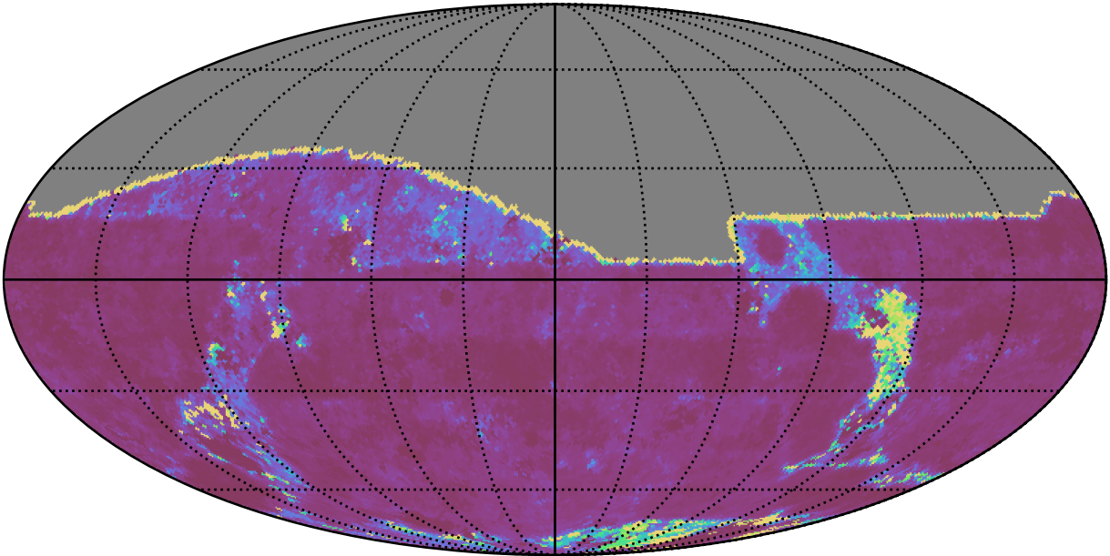
too_elab_heavy_r128_d3_ugrizy_v3.4_10yrs All sky g band: Median Inter-Night Gap
