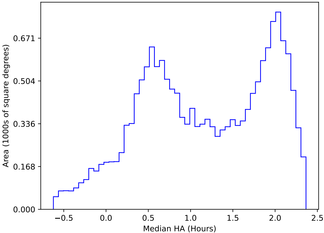
too_elab_heavy_r128_d3_ugrizy_v3.4_10yrs WFD z band: Median HA
