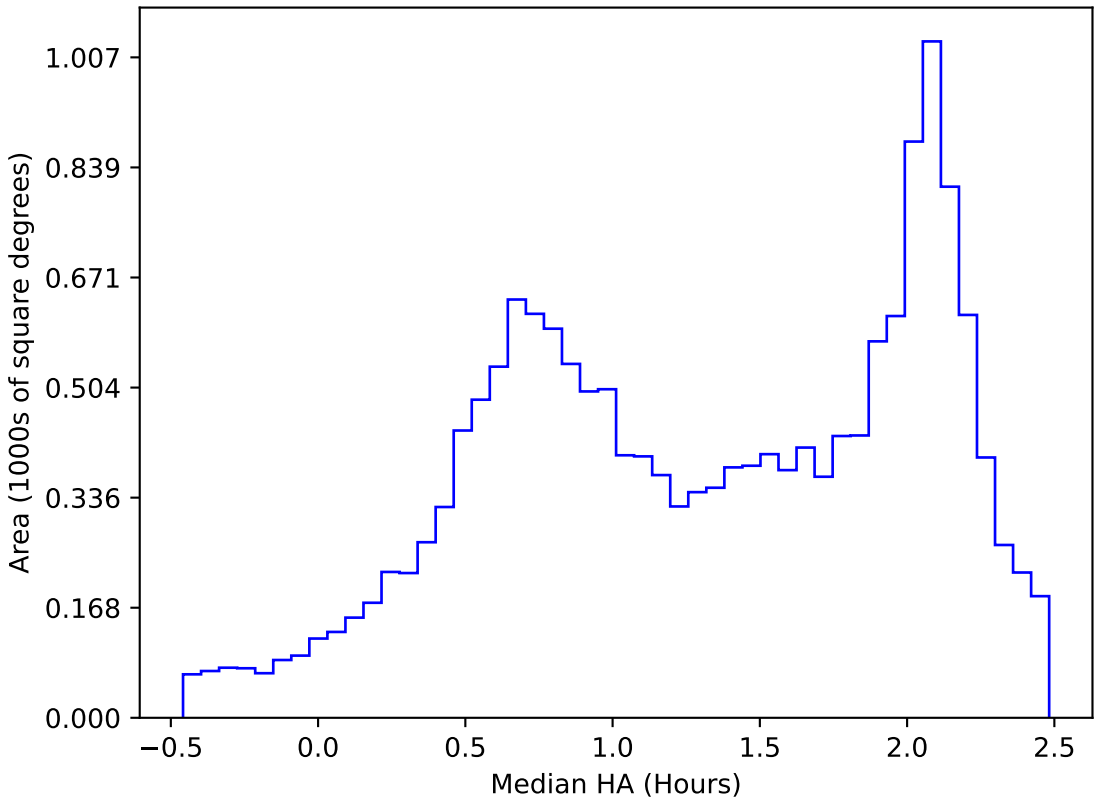
too_elab_heavy_r128_d3_ugrizy_v3.4_10yrs WFD y band: Median HA
