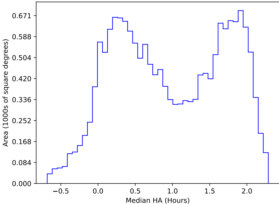
too_elab_heavy_r128_d3_ugrizy_v3.4_10yrs WFD r band: Median HA
