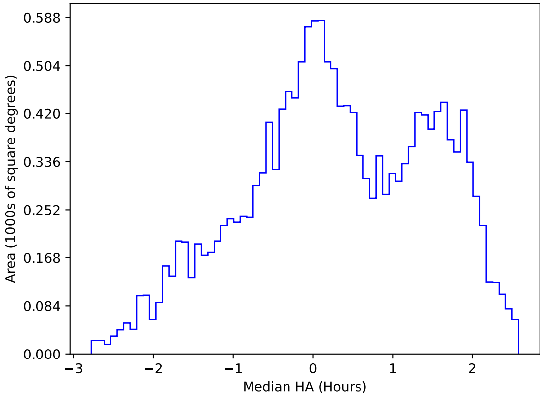
too_elab_heavy_r128_d3_ugrizy_v3.4_10yrs WFD g band: Median HA
