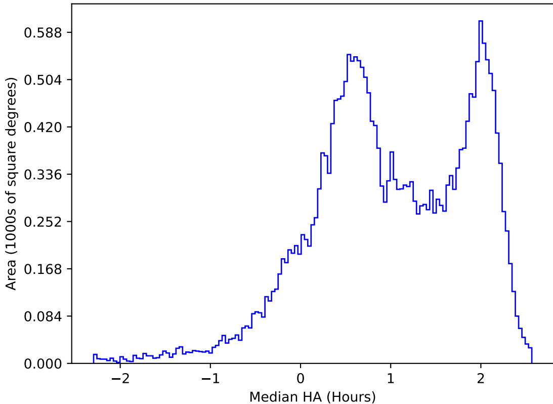
too_elab_heavy_r128_d3_ugrizy_v3.4_10yrs All sky z band: Median HA
