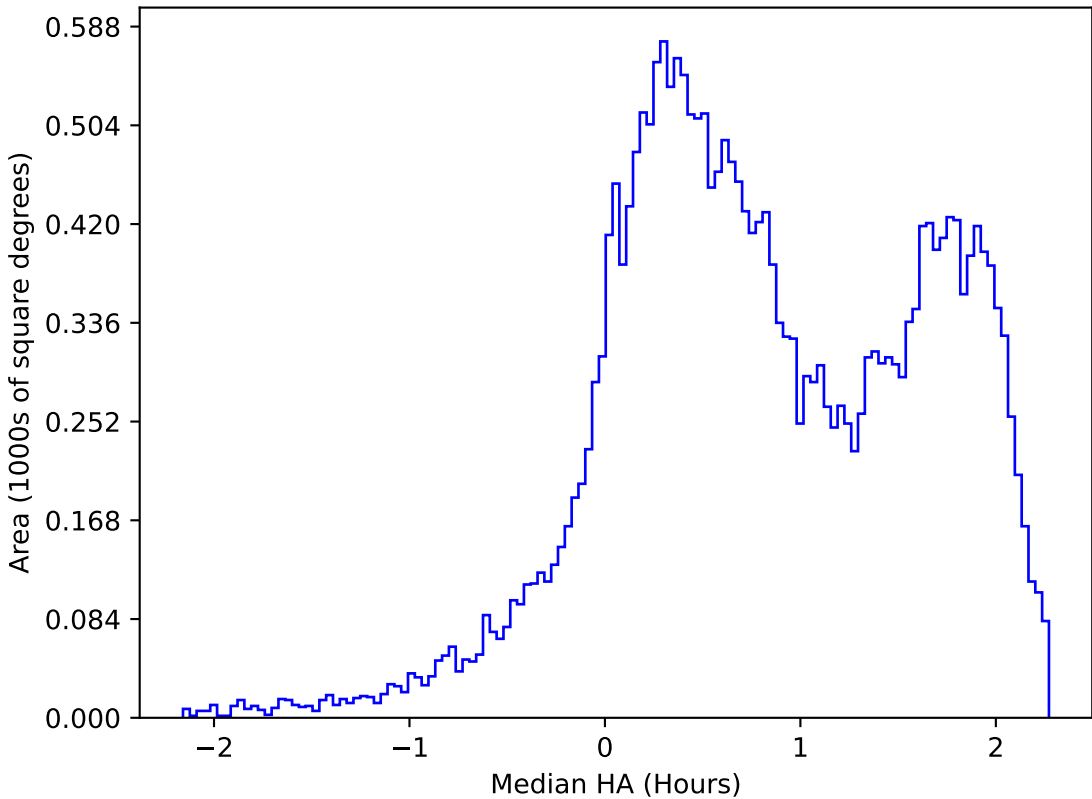
too_elab_heavy_r128_d3_ugrizy_v3.4_10yrs All sky r band: Median HA
