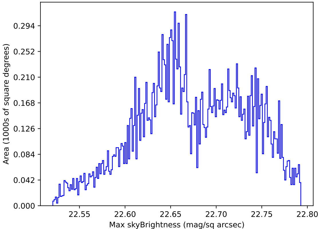
too_elab_heavy_r128_d3_ugrizy_v3.4_10yrs Yr 1 u band: Max skyBrightness
