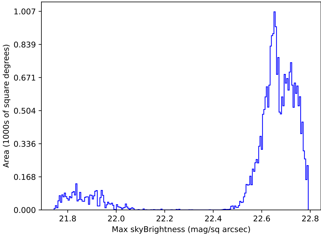
too_elab_heavy_r128_d3_ugrizy_v3.4_10yrs Yr 1 all bands: Max skyBrightness
