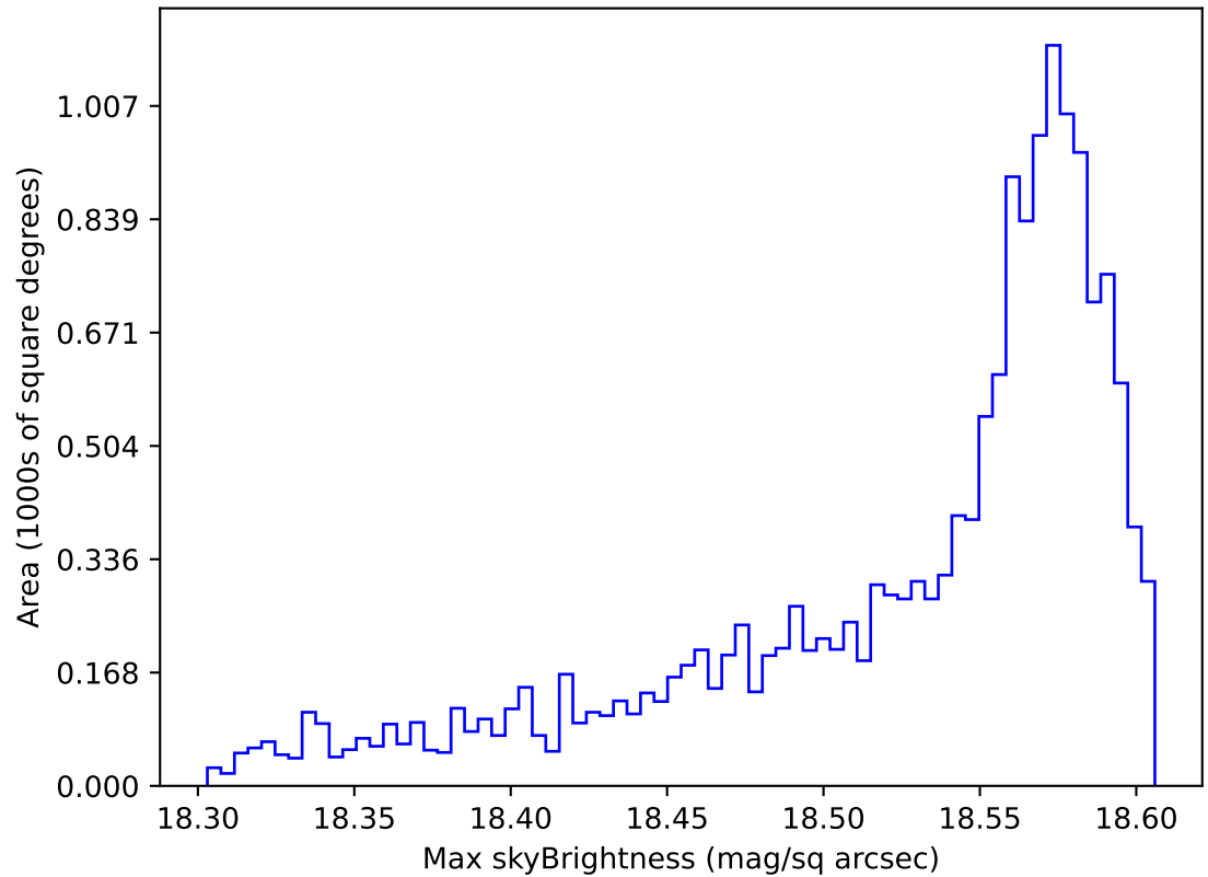
too_elab_heavy_r128_d3_ugrizy_v3.4_10yrs WFD y band: Max skyBrightness
