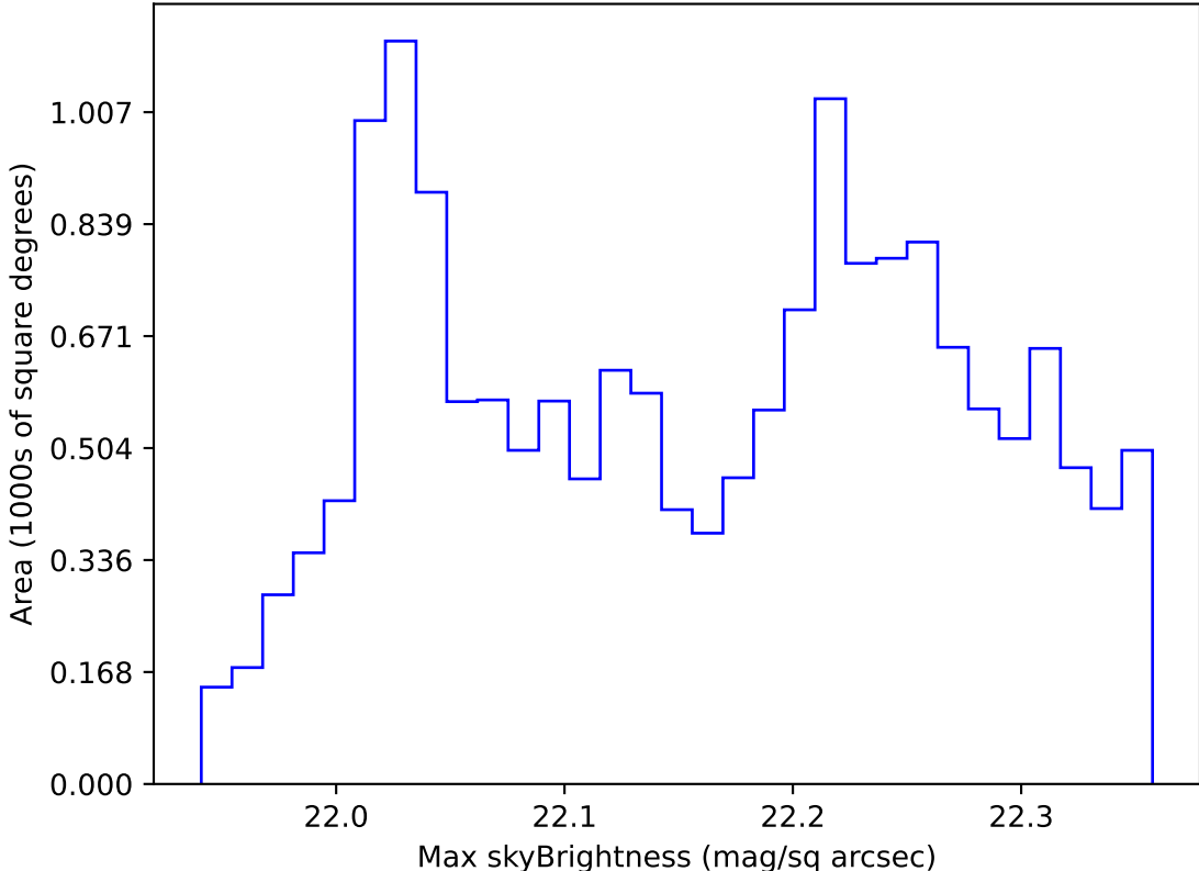
too_elab_heavy_r128_d3_ugrizy_v3.4_10yrs WFD g band: Max skyBrightness
